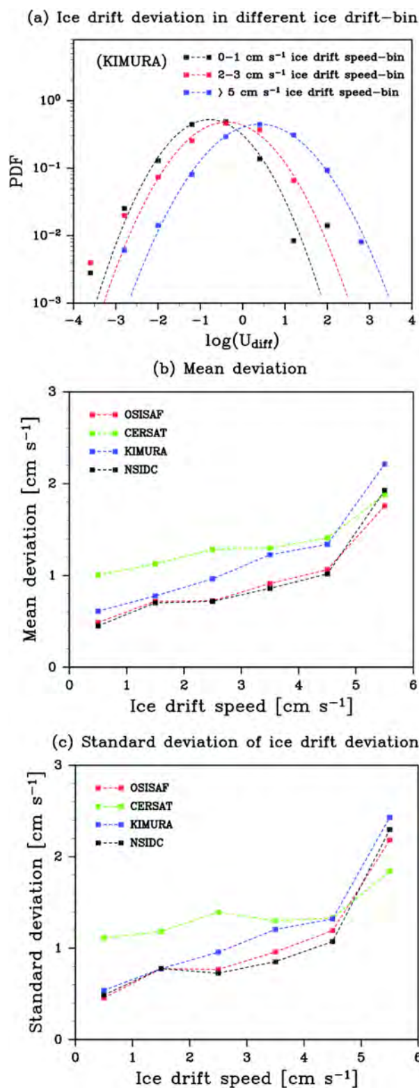
Figure 23. (a) Examples of distributions of ice drift deviation from monthly mean IABP/C drift in three ice drift speed bins (black: 0–1 cm s -1 , red: 2–3 cm s -1 , blue: > 5 cm s -1 ) for KIMURA. (b) Mean deviation and (c) standard deviation from monthly mean IABP/C drift estimated from the corresponding lognormal distribution.
