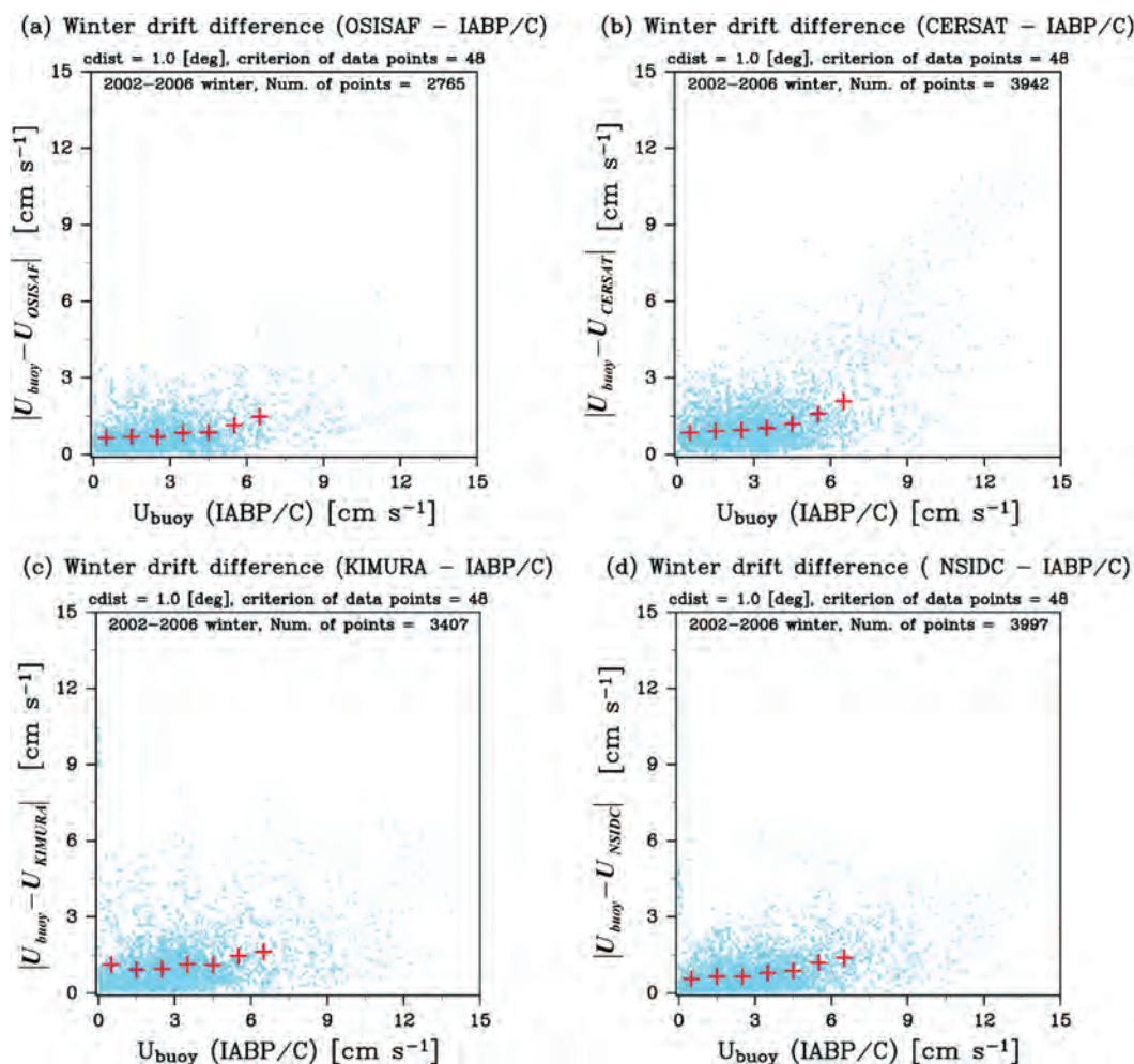
Figure 19. Scatter plot of ice drift difference between satellite-derived and IABP/C buoy data as a function of buoy drift speed: (a) OSISAF, (b) CERSAT, (c) KIMURA, and (d) NSIDC. Ice drift data in winter (November to April) from 2002 to 2006 were used to plot the points. Each light-blue point denotes difference of ice drift at a certain grid point. The red crosses denote the mean difference of ice drift in a certain bin ( 1.0 \text{ cm s}^{-1} width) of IABP/C buoy drift speed.
